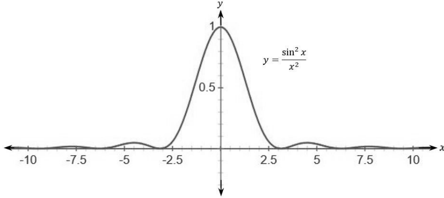
Figure 3: Plot of \sin^2(x)/x^2 .
