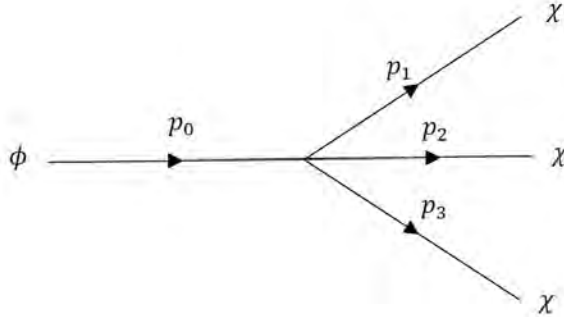
Figure 1: First order process in \phi\chi^4 interaction.
