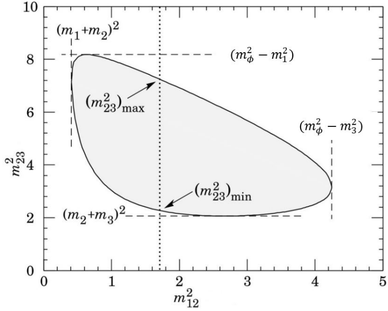
Figure 2: Dalitz plot. Produced from [5]
