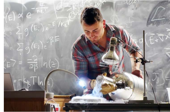
The Meissner Effect!
