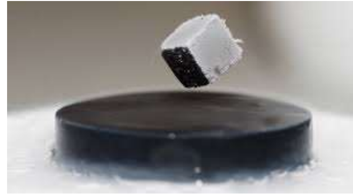
The Meissner Effect!
